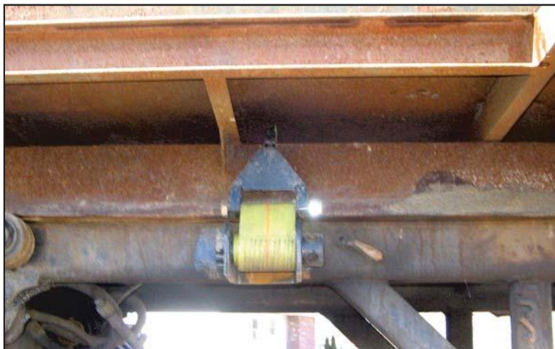
Waste/Rolloff Container - Style 2 (Webbing may be changed in the field) Part No. 87A3235001
