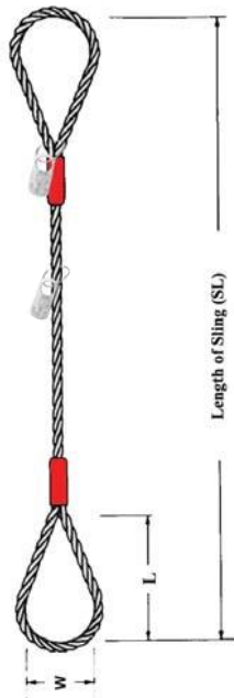
Single Leg Redi-Grip® Sling
